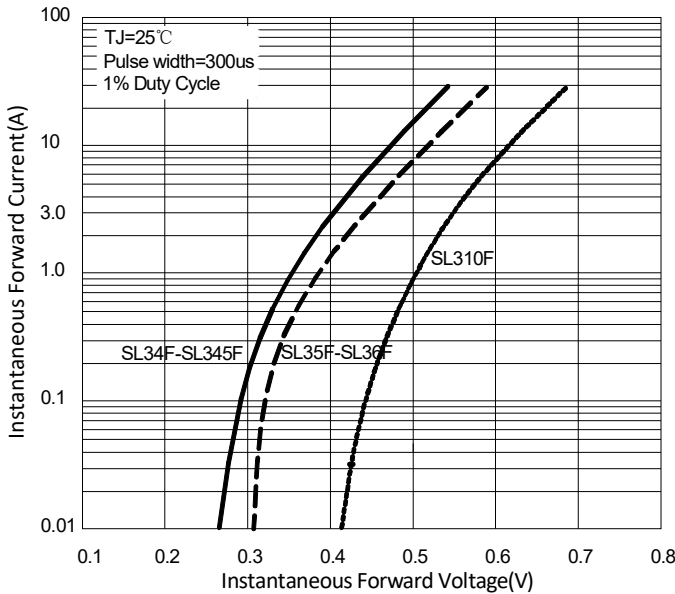
FIG3: Forward Voltage
